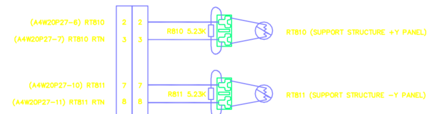
W19 SUPPORT STRUCTURE THERMISTORS (ASSY 36-30123)
