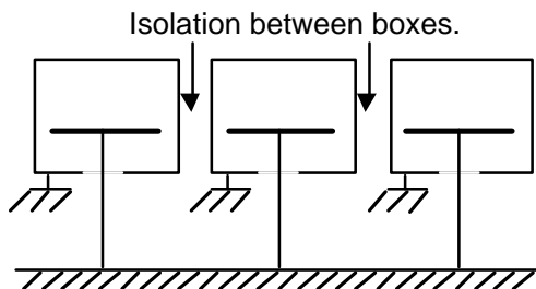
FIGURE 6. Multiple, Single Reference Ground System
