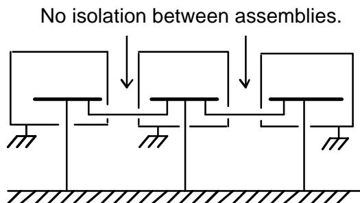
FIGURE 5. Multiple-Point Ground
