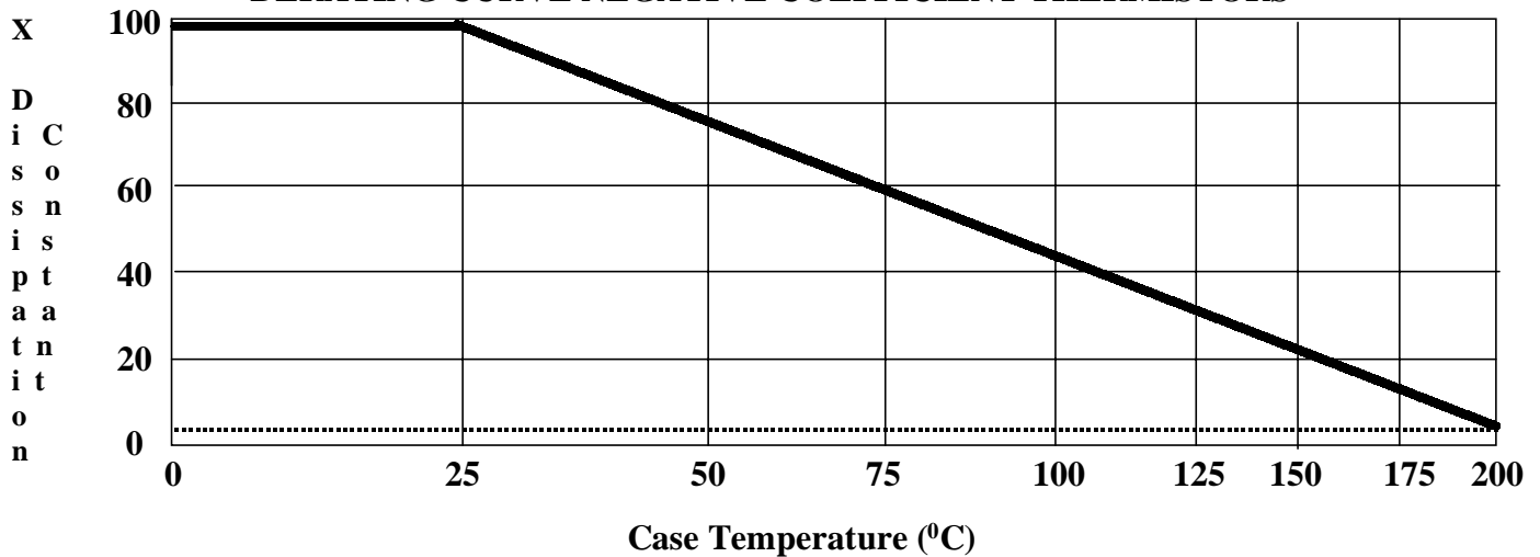
DERATING CURVE NEGATIVE COEFFICIENT THERMISTORS
