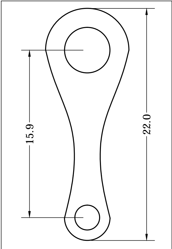
PART BEFORE BENDING
