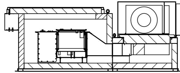
SECTION F-F SCALE 1 : 20
