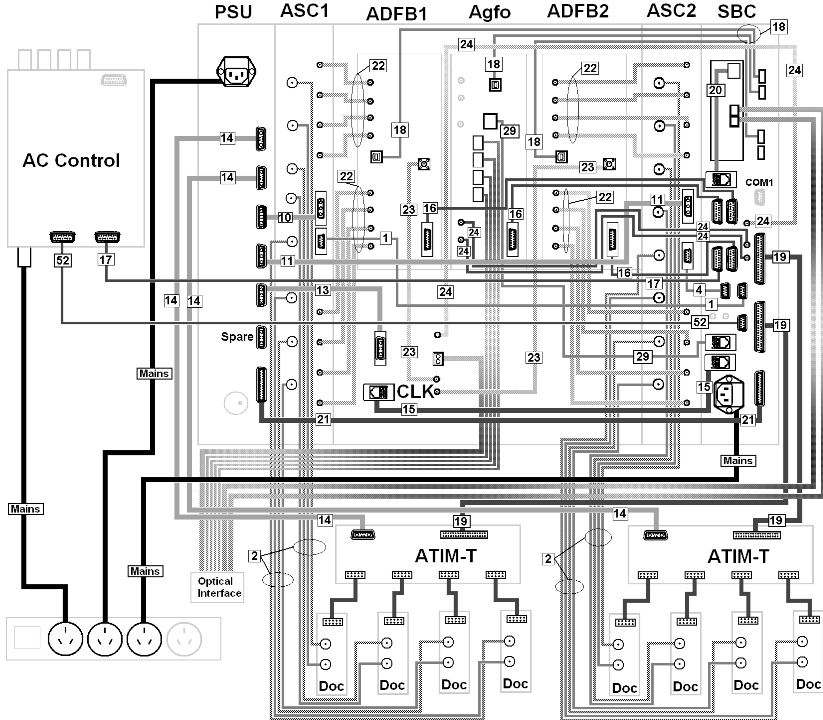
Enclosure Wiring Cable Diagram
