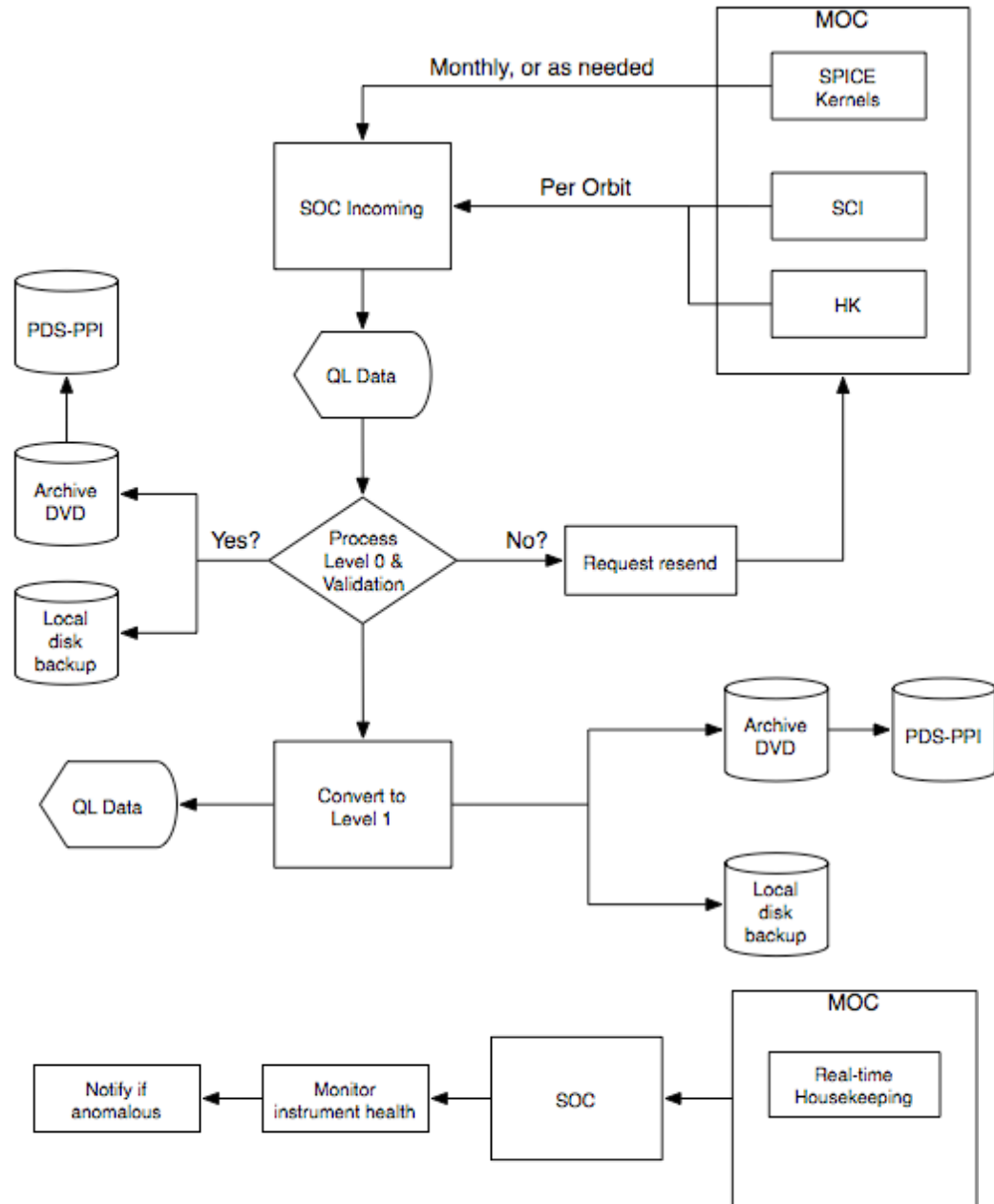
Figure 3-1 SOC Interfaces
