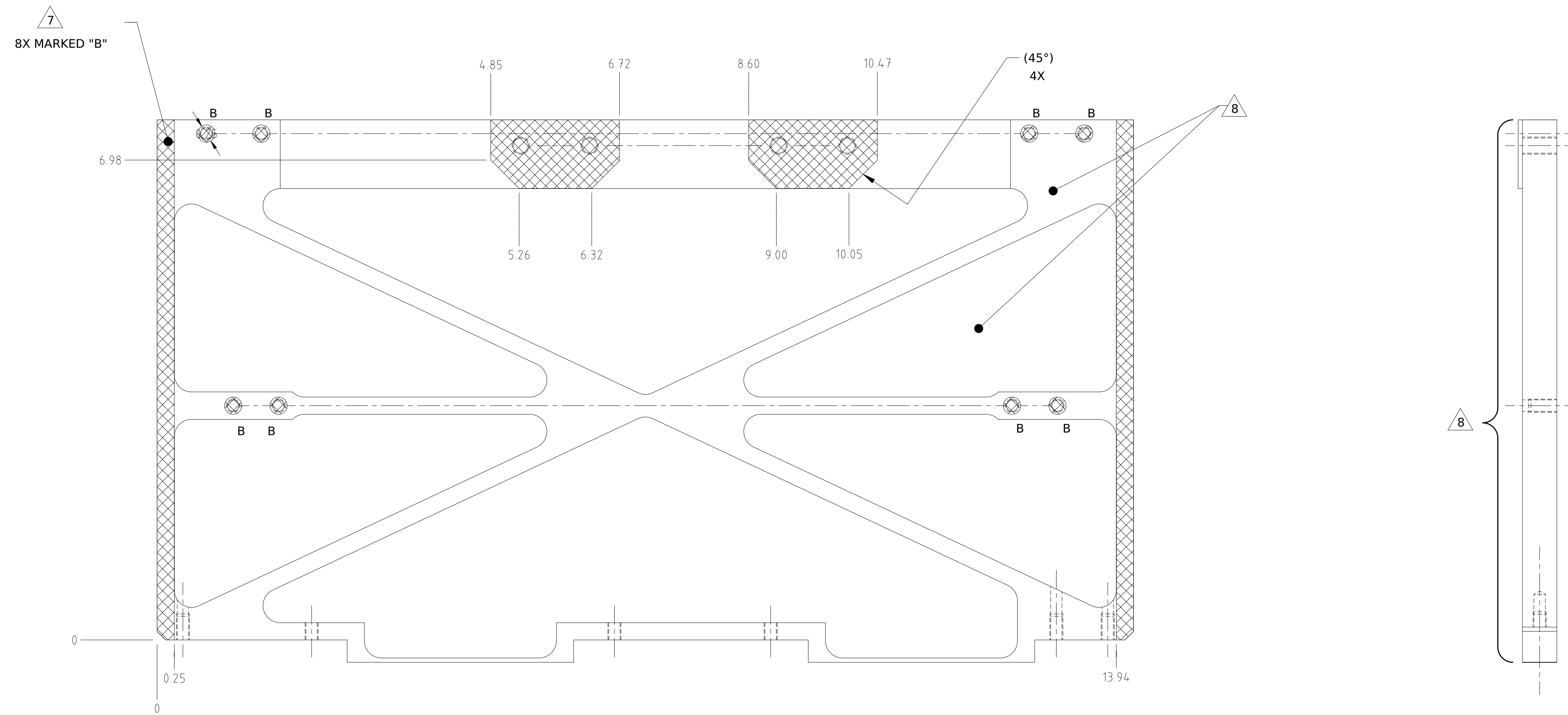
MASKING DETAIL
