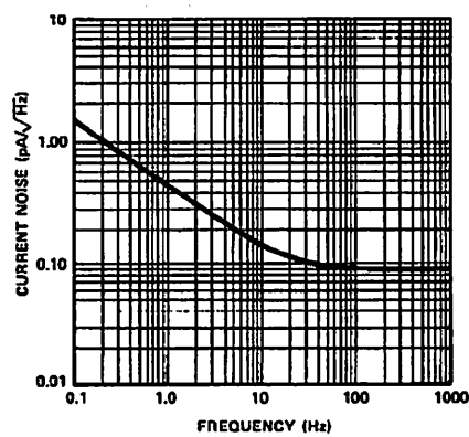
CURRENT NOISE DENSITY ( i_n ) vs FREQUENCY
