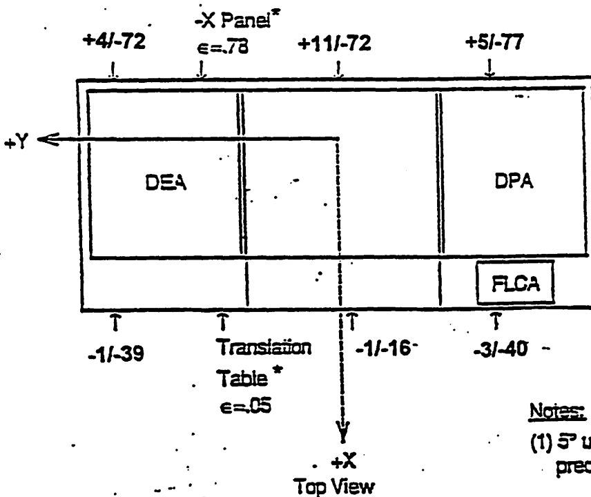
Figure 3.3-1: ISIM Hot and Cold Operational Case Boundary Temperatures and IR Emittances for ACIS Detector Cables and ACIS Proton Shield/DPA/DEA Thermal Analysis
