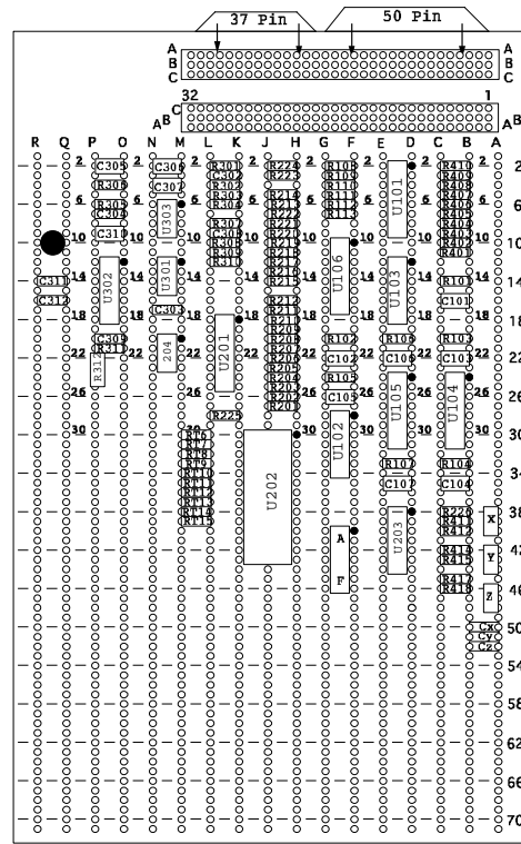
Wire Side
