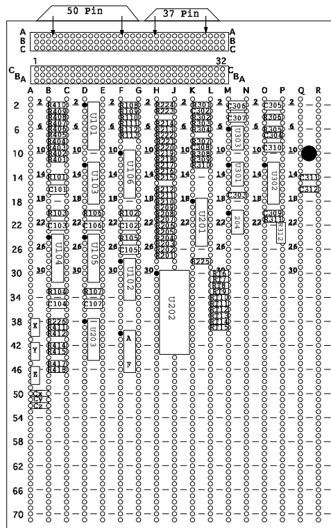
Component Side
