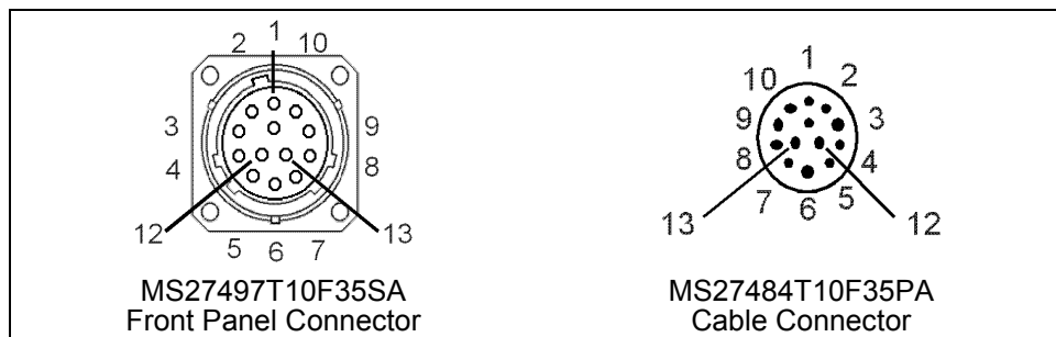
Figure 3-7. IRIG-B Connector Face
