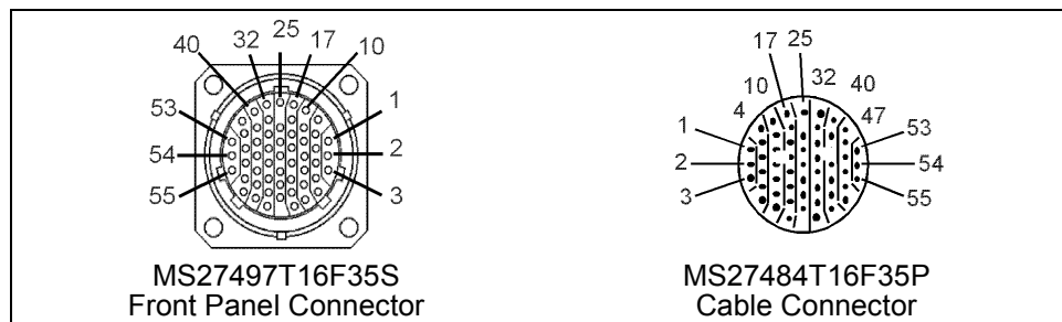
Figure 3-8. CD/DVD Connector Face
